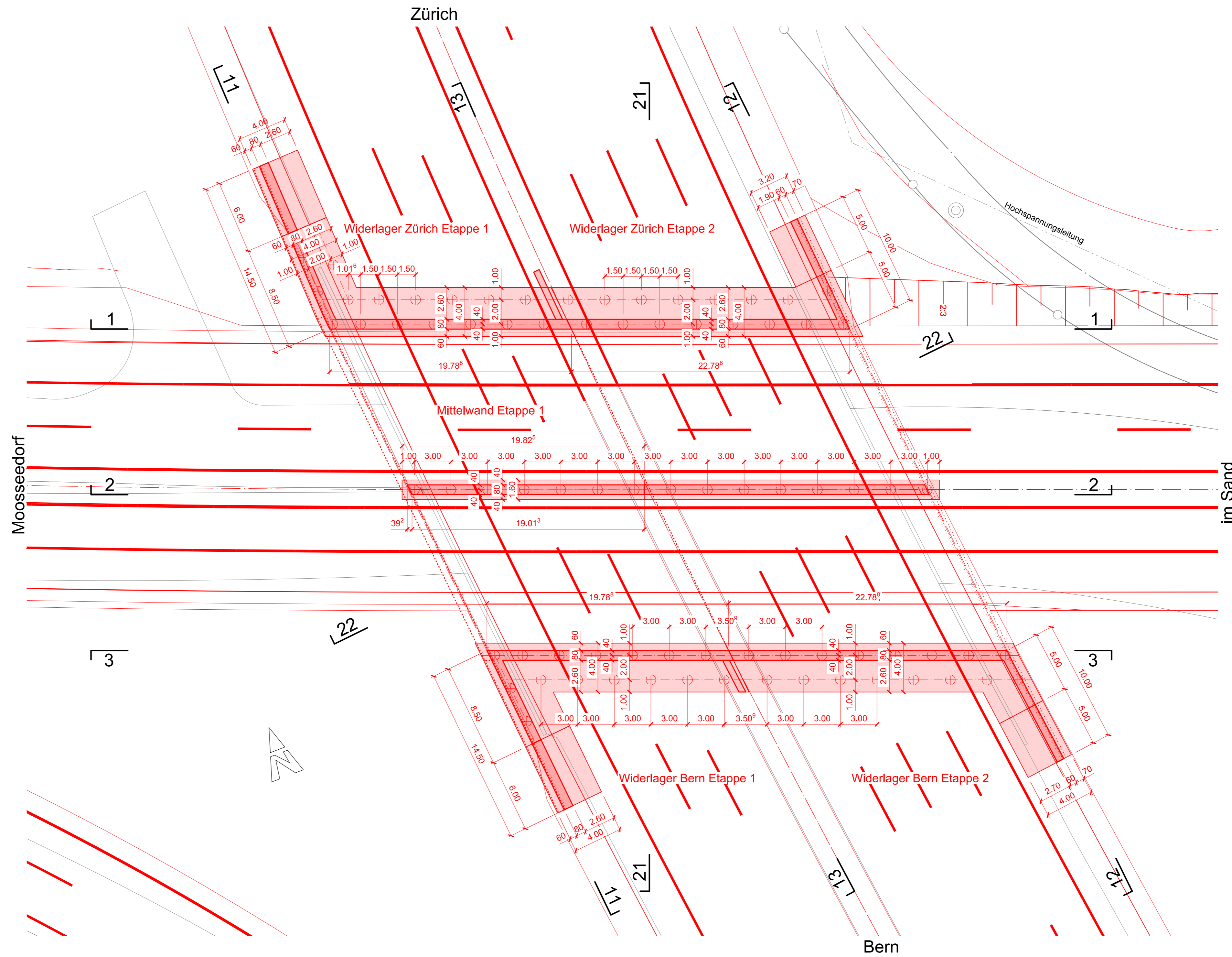
Situation Fundation 1:200
